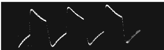
Square Wave Distortion from poor response at both low and high frequency. (A typical amplifier oscillogram.)
